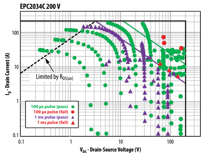
Figure 19: EPC2034C SOA plot. The “Limited by R_{DS(on)} ” line is based on data sheet maximum specification for R_{DS(on)} at 150°C. Measurements for 1 ms (purple triangles) and 100 \mu s (green dots) pulses are shown together. Failures are denoted by red triangles (1 ms) or red dot (100 \mu s). Note that all failures occur outside the data sheet SOA region.
