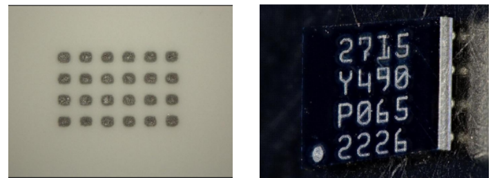
Figure 31: (Left) Solder stencil pattern squeezed onto ceramic substrate. (Right) EPC2715 after reflow onto substrate.
