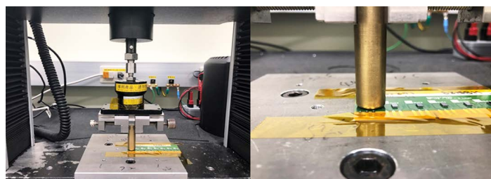
Figure 27: Pressure test instrument. The tester head lowers to the backside of the devices using a constant loading speed of 0.6 mm/min until the predetermined force is sensed by the gauge. The DUTs are surface mounted on a FR4 test coupon that is secured on the testing stage.
