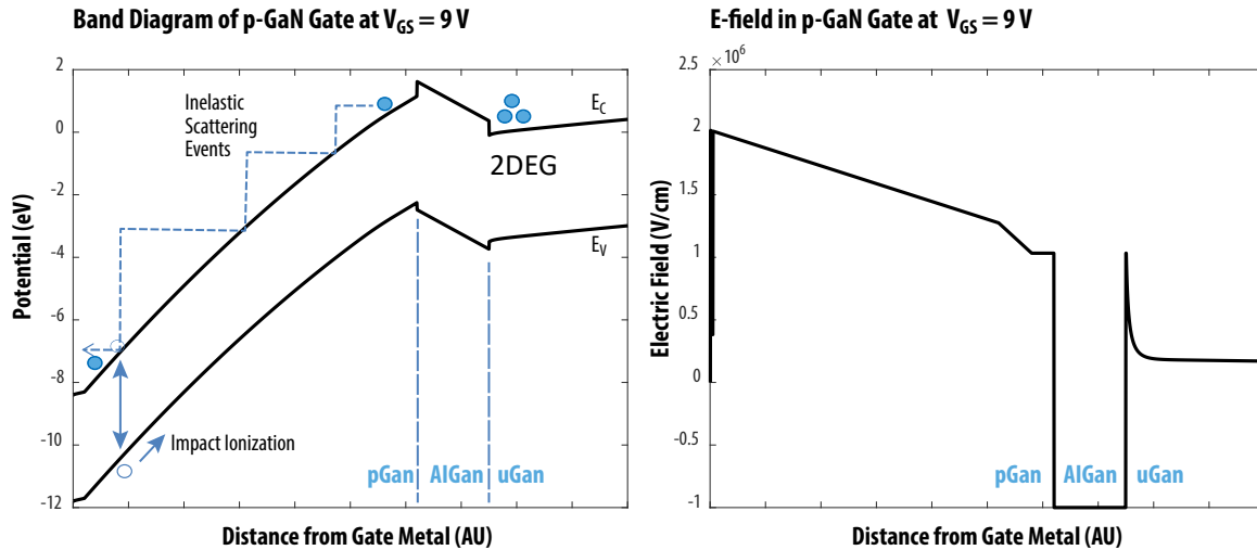
Figure A2: (Left) Band-diagram of eGaN gate under high forward bias (9 V). Far left corresponds to the gate metal; AlGaIn front barrier is seen toward the right. Note that electron-hole pair production is depicted in the high field region near the gate metal. (Right): Electric field in the gate for the same conditions. Note the field is not uniform, reaching a peak > 2 MV/cm
