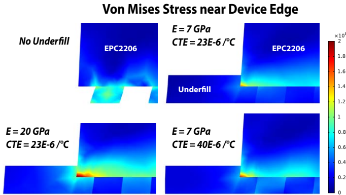
Figure 37: Von Mises (peak shear stress) in the edge-most solder bar under a temperature cycle change of \Delta T = +100^\circ\text{C} . Four different underfill conditions are simulated, with changing Young's modulus ( E ) of the underfill and different CTE as well. Note that deformation has been exaggerated by the same scale in each picture.
