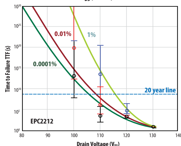
Figure 7: The data in Figure 4, as well as similar data taken at different temperatures, is translated into predictions of failure rates over time, temperature, and voltage.
