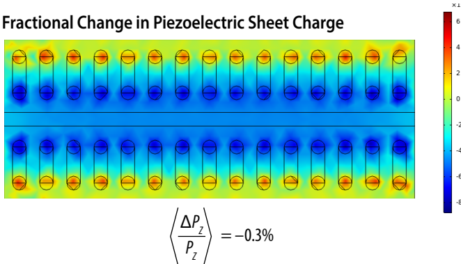
Figure 30: Fractional change in piezoelectric sheet charge for an EPC2206 under strain from 4 mm board deflection. The area averaged change in piezoelectric charge is less than -0.3\% , while the peak change is around 0.8\% in the immediate vicinity of solder bars. These changes in piezoelectric polarization are too small to create observable changes in device parameters V_{TH} or R_{DS(on)} .
