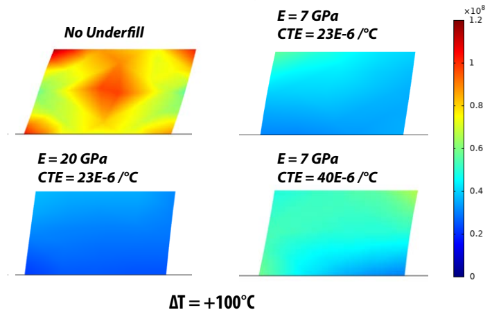
Figure 36: Von Mises (peak shear stress) in the edge-most solder bar under a temperature cycle change of \Delta T = +100^\circ\text{C} . Four different underfill conditions are simulated, with changing Young's modulus ( E ) of the underfill, and different CTE as well. Note that mechanical deformation has been exaggerated by 20x in all cases.
