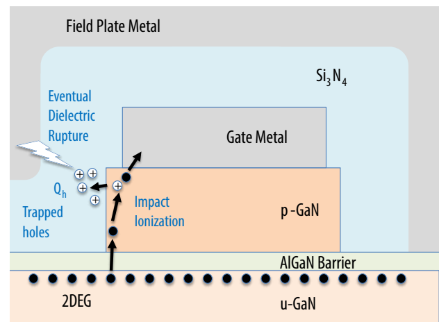
Figure A1: Schematic of gate failure mechanism in an eGaN FET. A small current of electrons tunneling through the AlGaN front barrier enter the p-GaN gate region, where they are accelerated in high fields toward the gate metal. A small percentage gain sufficient energy to cause impact ionization, particularly near the gate metal. The resulting holes are mostly swept away, but some trap and accumulate in the \text{Si}_3\text{N}_4 dielectric layer. Once sufficient trapped hole density, Q_h , has accumulated, fields concentrate in the dielectric, ultimately leading to catastrophic rupture.
