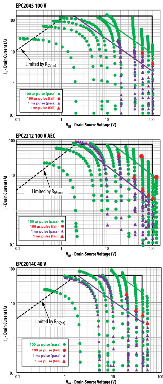
Figure 20: SOA results for EPC2045, EPC2212, EPC2014C. Measurements for 1 ms (purple triangles) and 100 \mu s (green dots) pulses are shown together. Failures are denoted by red triangles (1 ms) or red dot (100 \mu s). Note that for all parts, all failures occur outside the data sheet SOA region.
