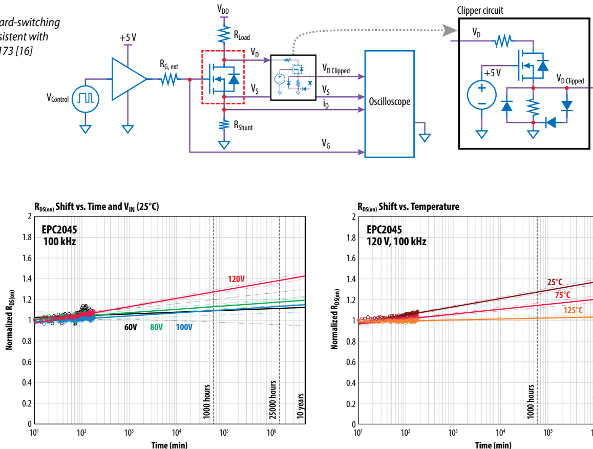
Figure 10: The R_{DS(on)} of a fifth-generation EPC2045 eGaN FET over time at various voltage stress levels and temperatures. On the left, the devices were tested at 25°C at voltages from 60 V to 120 V. The graph on the right shows the evolution of R_{DS(on)} at 120 V at various temperatures.
